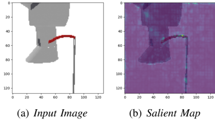
Fig. 7. The input image of the actor network and the corresponding salient map from the actor network
