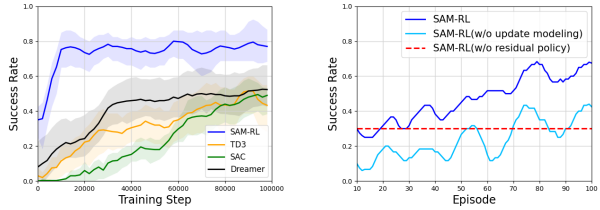
(c) Comparison with model-free and model-based RL in simulation on Needle-Threading (d) Ablation studies in real world on Needle-Threading
