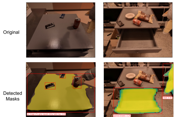
Fig. 5: We show the original images from RT-1 datasets on the top row and the images with detected masks and mask labels on the bottom row.
