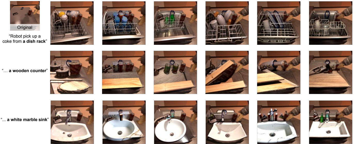
Fig. 6: We show visualizations of the episodes generated by ROSIE where we replace the regular tabletop in front of the robot with a dish rack, a marble sink and a wooden counter, which never appears in the training dataset. Our results in Section V-A and Figure 7 show that the policy trained on such augmentations enables the robot to place objects into a real metal sink.
