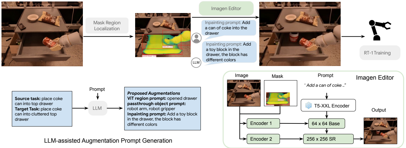
Fig. 2: The proposed architecture of ROSIE. First, we localize the augmentation region with open vocabulary segmentation model. Second, we run Imagen Editor to perform text-guided image editing. Finally, we use the augmented data to train an RT-1 manipulation policy [4]. Concretely, we explain ROSIE using the example shown in the figure as follows. We take the original episode with the instruction “place coke can into top drawer” and the goal is to add distractors in the opened drawer to improve the robustness of the policy. For each image in the episode, we detect the masks of the open drawer, the robot arm, and the coke can using our first step. We obtain the mask of the target region to add the distractor via subtracting the masks of the robot arm and the coke can that is picked up from the mask of the open drawer. Then, we generate our augmentation proposal leveraging LLMs as described in Section IV-B. We run Imagen Editor with the augmentation text and the selected mask to generate a coke can in the drawer discussed in Section IV-C. We combine both the original episodes and the augmented episodes and perform policy training using multi-task imitation learning.
