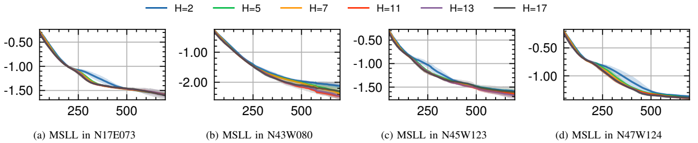
Fig. 15. Sensitivity analysis of the choice of H .
