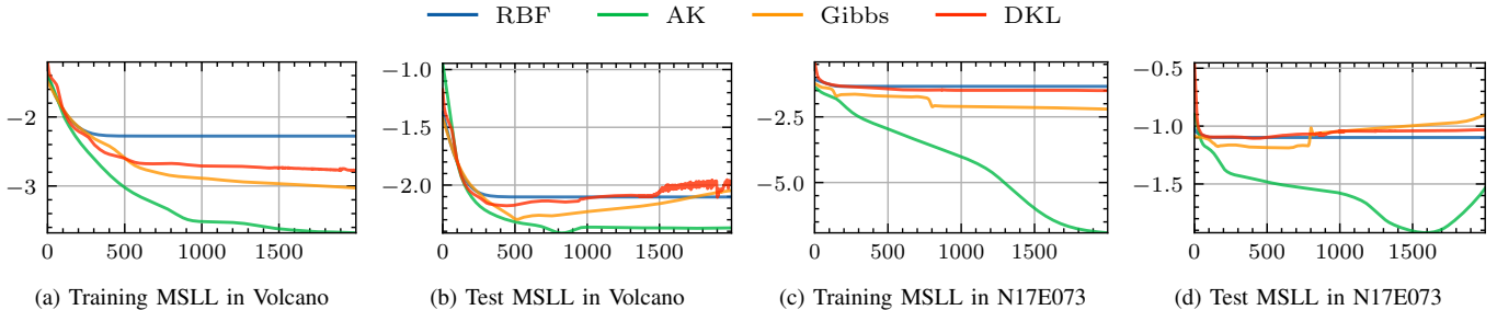
Fig. 19. Results of the overfitting analysis in the Volcano environment introduced in Fig. 1a and N17E073.
