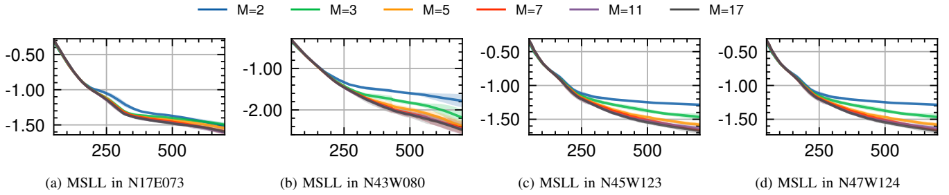
Fig. 14. Sensitivity analysis of the choice of M .
