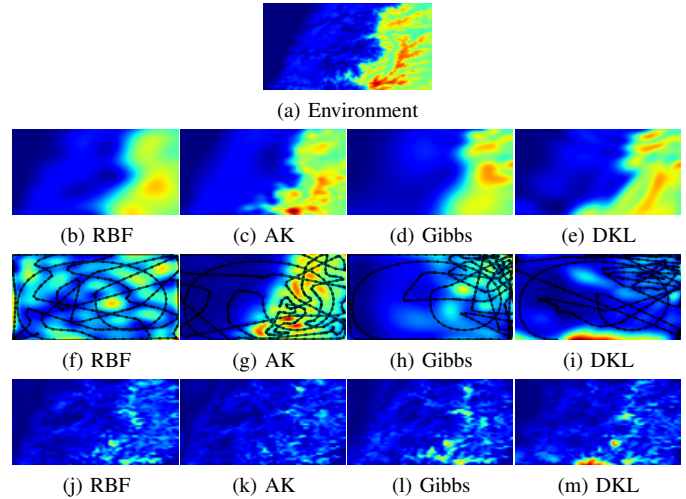
Fig. 11. Snapshots of RIG with different kernels. (b-e) show the prediction maps, (f-i) are the uncertainty maps with sampling paths, and (j-m) present the absolute error maps.
