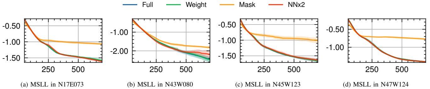
Fig. 18. Results of the four variants in the ablation study.
