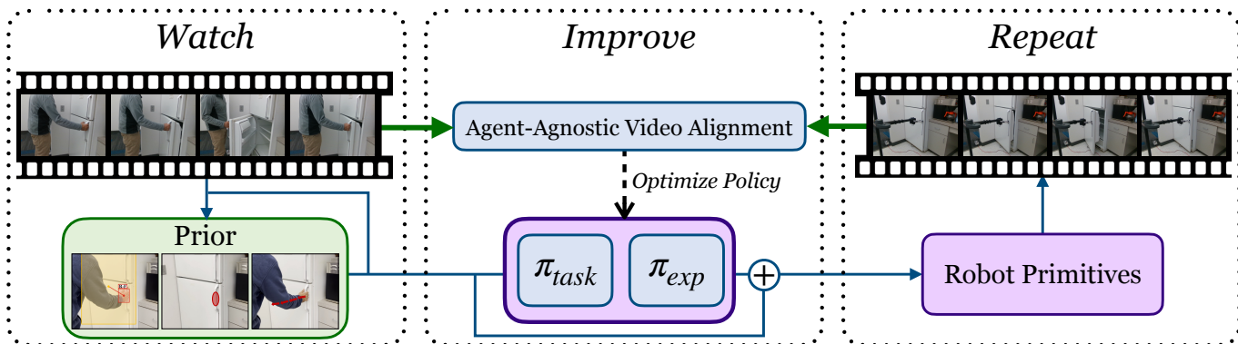
Fig. 2: Our method (WHIRL) provides an efficient way to learn from human videos. We have three core components: we first “watch” and obtain human priors such as hand movement and object interactions. We “repeat” these priors by interacting in the real world, by both trying to achieve task success and explore around the prior. We “improve” our task policy by leveraging our agent-agnostic objective function which aligns human and robot videos.
