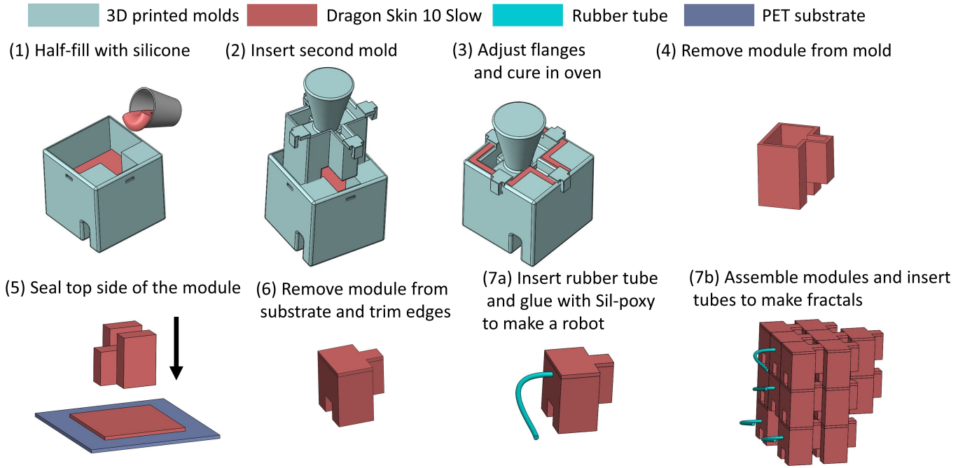
Fig. 5. Manufacturing fractal robots. (1) 3D printed mold was partially filled with Dragon Skin 10 Slow and then placed in a vacuum oven to degas for 5 minutes. (2) Second 3D printed mold was inserted into the first mold slowly to avoid introducing air bubbles into the silicone. (3) Flanges on the second mold were adjusted on the first mold to keep a 2 mm clearance between the walls of the molds. Silicone was cured in the oven at 60°C for 75 minutes. (4) The module was removed from the mold and the edges were trimmed. (5) The module was flipped over an uncured layer of silicone and its top side was sealed. (6) The module was removed from the substrate and its edges were trimmed. (7a) A hole was punched in one of the sides of the module and a rubber tube was inserted and glued using Sil-poxy as the bonding agent to make a robot (video). (7b) Basal robots join together to form a fractal robot (video).
