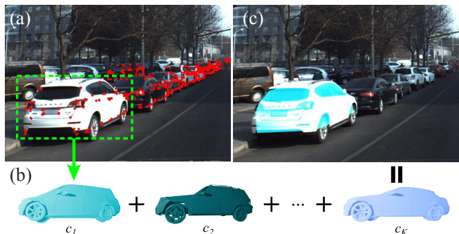
Fig. 1: We propose the first certifiably optimal approach to estimate the 3D pose and shape of objects from 3D keypoint detections (red points in (a)). Our approach estimates pose and shape using an overcomplete library of CAD models (b) and is robust to up to 70–90% outliers in the detections. (c) The approach is more accurate than the state of the art on the ApolloScape dataset [80].
