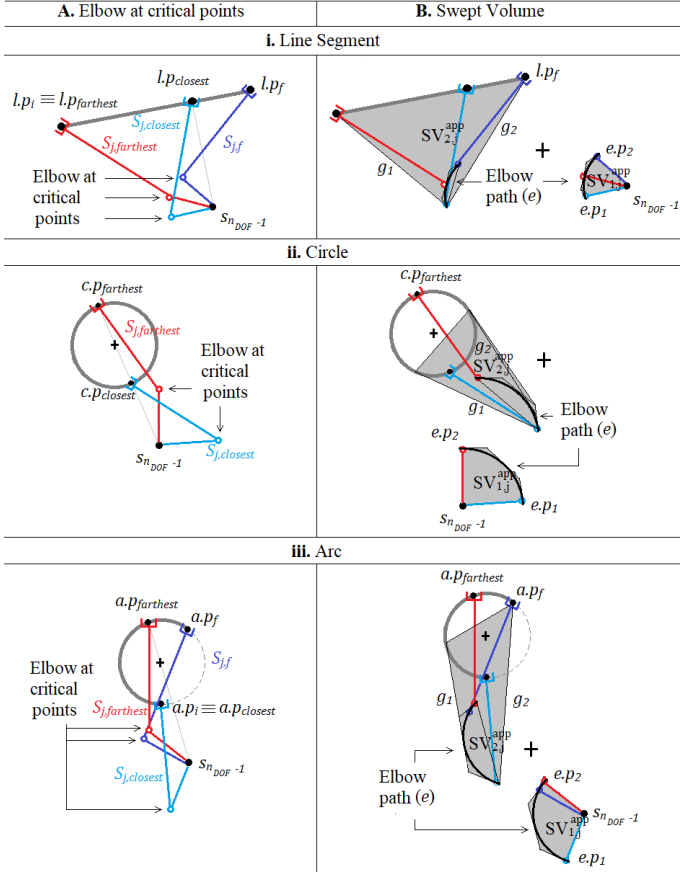
Fig. 4: SV_j^{app} construction. We do not allow obstacles inside circles or arcs defined by arcs. (A) Elbow position at critical points and (B) swept volume for a line segment (i), a circle (ii) and an arc (iii). Critical states are in dark blue ( S_{j,f} ), light blue ( S_{j,closest} ) and red ( S_{j,farthest} ). The SV is decomposed into the SV of the n_{DOF}-1 link, a pentagon over approximation of a sector, and the n_{DOF} link, the convex hull of the elbow and EE boundary positions.
