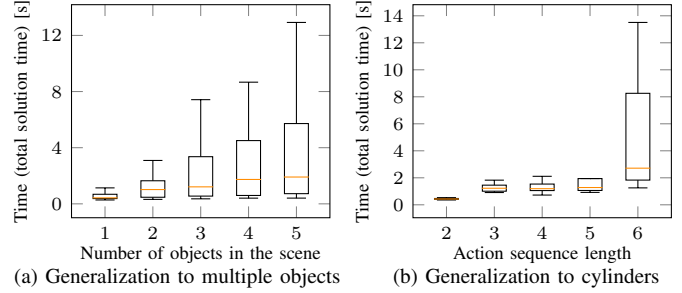
Fig. 7. Generalization experiments.
