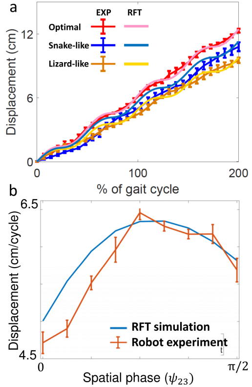
Fig. 5. Robot experiment and RFT simulation results (a) The primary data of displacement from robot experiments (solid lines with error bars) and RFT simulation (solid lines) plotted as a function of gait percentage over two gait cycles for snake-like body undulation (blue), optimal body undulation (red) and lizard-like body undulation (yellow). (b) The displacement is plotted as a function of spatial phase. The red curve with error bars shows the robot experiment results. The blue curve shows the RFT simulation results.
