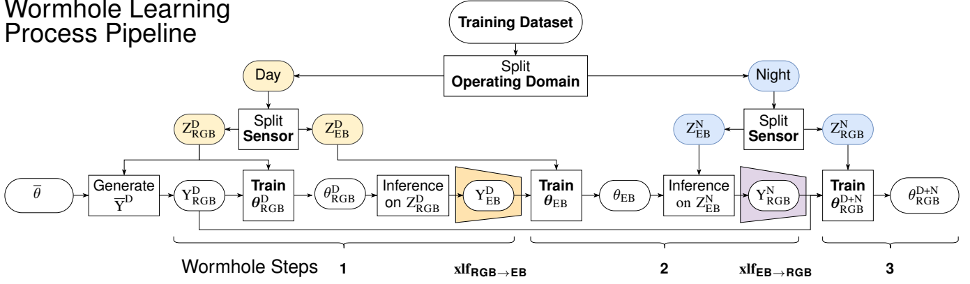
Fig. 8. The process can be generally divided into three sub-tasks: 1) Training of the network using day-time only annotations and transferring generated labels to OD_{EB} , after it has been passed through the cross-modal learning filter ( xlf_{RGB \rightarrow EB} ), depicted as orange funnel. 2) Training of the event-based network using labels generated by the object detector trained in last step and exploiting invariance of the DVS camera to generate labels at night, which are transferred back to OD_{RGB} . Here, the violet funnel represents the cross-modal learning filter ( xlf_{EB \rightarrow RGB} ) from EB to RGB. 3) Wormhole loop is closed by retraining the original network with day-time and night-time data from the event-based network.
