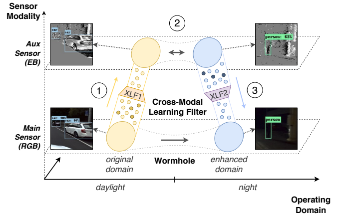
Fig. 1. The principle of wormhole learning is illustrated. Starting from the bottom left, in a first step, transfer learning is applied to learn a detector in the auxiliary domain. From there, the inherent invariance to a specific nuisance for the task allows us to travel across the operating domain. In the final step, the loop is closed performing another domain transfer: back into the main sensor space, but in a new operating envelope. We validate this concept adopting an event-based camera (EB) as auxiliary sensor and exploiting its inherent invariance to illumination, we can enhance the main RGB detector. With the due carefulness, the principle still applies even though the two sensors are radically different. Indeed, we have to introduce two cross-modal learning filters (XLFs) to cope with the, otherwise “noisy”, domain transfer steps.
