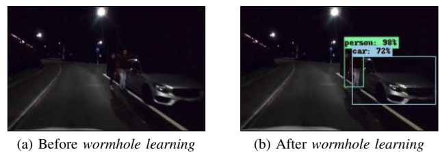
Fig. 2. Despite the availability of labeled data only for daytime, wormhole learning successfully improved RGB object detection performance in insufficiently illuminated environments. Take, for instance, a parked car on the curb without headlights. At night it has a different appearance than at day (e.g. no reflections on the windows), yet is detected after wormhole learning.
