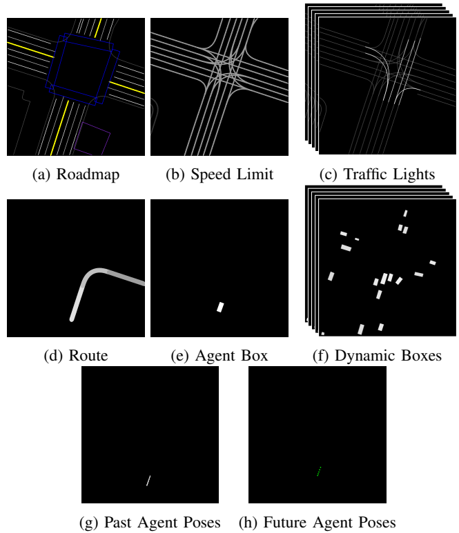
Fig. 2: Driving model inputs (a-g) and output (h).
