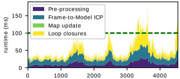
Fig. 7. Processing time needed to map sequence 00 from the KITTI Vision Benchmark. See Figure 1 for the finally registered complete point cloud.
