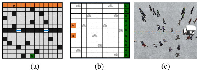
Fig. 3: Large-scale planning tasks for evaluating HyP-DESPOT. (a) Navigation with a partially known map. (b) Multi-agent rock sample. (c) Autonomous driving in a crowd.
