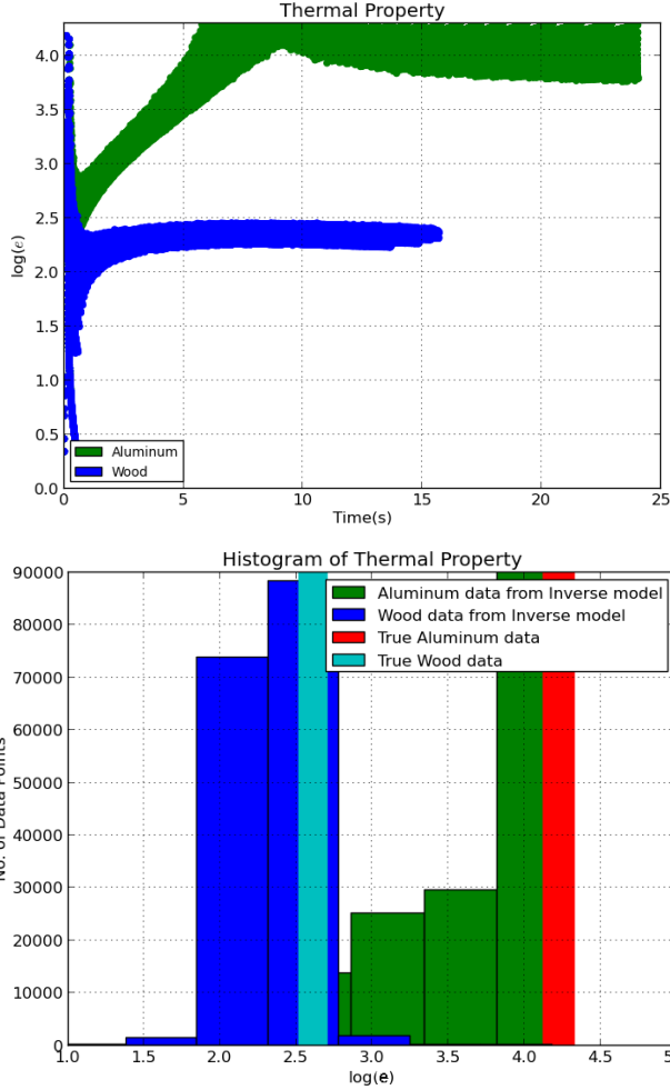
Fig. 9: Inverse Simulation of the heat-transfer data (top), Histogram of the thermal property (bottom). Shaded regions in the histogram show the true values.
