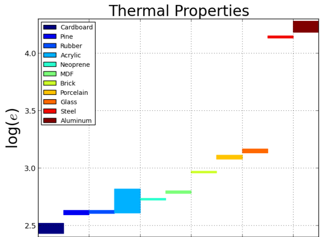
Fig. 10: Thermal properties of materials used for experiments. Each material has a minimum and maximum value for \log(e) . The values are taken from CES materials database [26].
