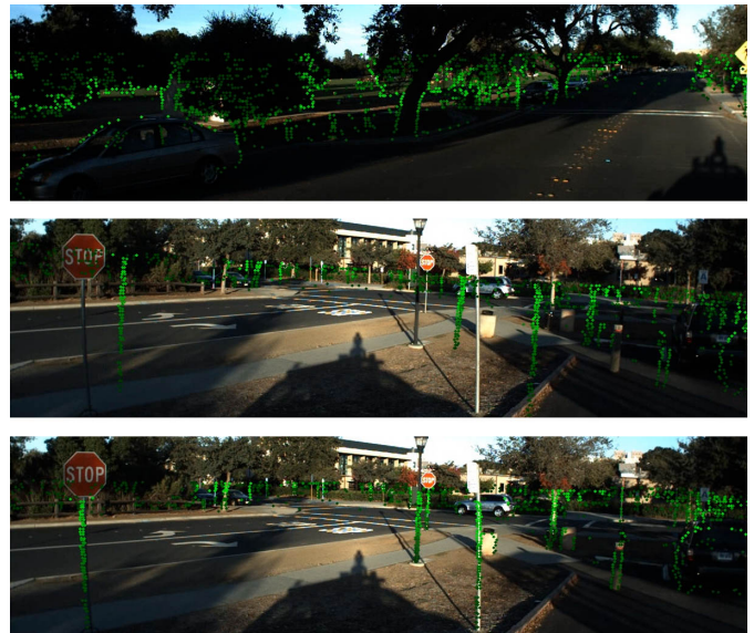
Fig. 9. Tracking calibration errors in real time. (Top) shows the first frame in a 400-frame sequence. Initially, the transform is correct. We then synthetically perturb two translation and two rotation parameters, over the course of the 400 frames, resulting in a badly miscalibrated sensor (Middle). However, with our online tracking algorithm, the transform updates itself in real time, adjusting to the perturbations, and ends up almost perfectly calculating the synthetic shift all the way through the end of the sequence (Bottom).
