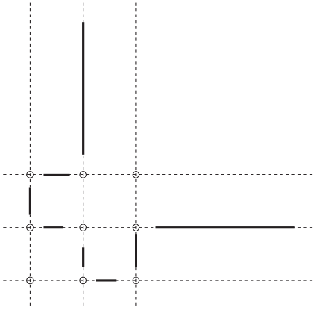
Fig. 5. An overhead view of a floor plan of the scene indicating the walls, which are considered to have infinite extent and are depicted by dashed lines, and the wall segments, which are depicted by the solid line segments. These wall segments correspond to contiguous planar regions in the RGB-D image. The interpretation system also considers all of the possible intersections between perpendicular walls, denoted by circles in the figure, since these may correspond to corners in the scene.
