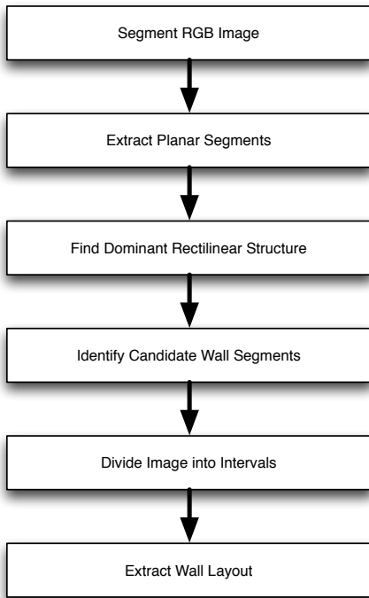
Fig. 2. Flowchart of overall parsing procedure.
