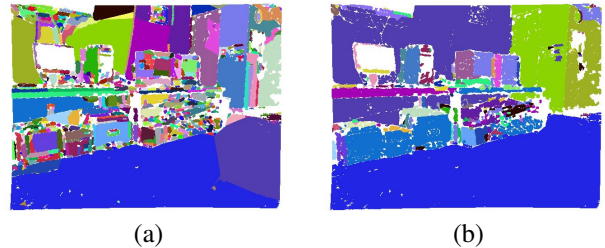
Fig. 4. a. Extracted Planes b. Result after coplanar segments are merged
