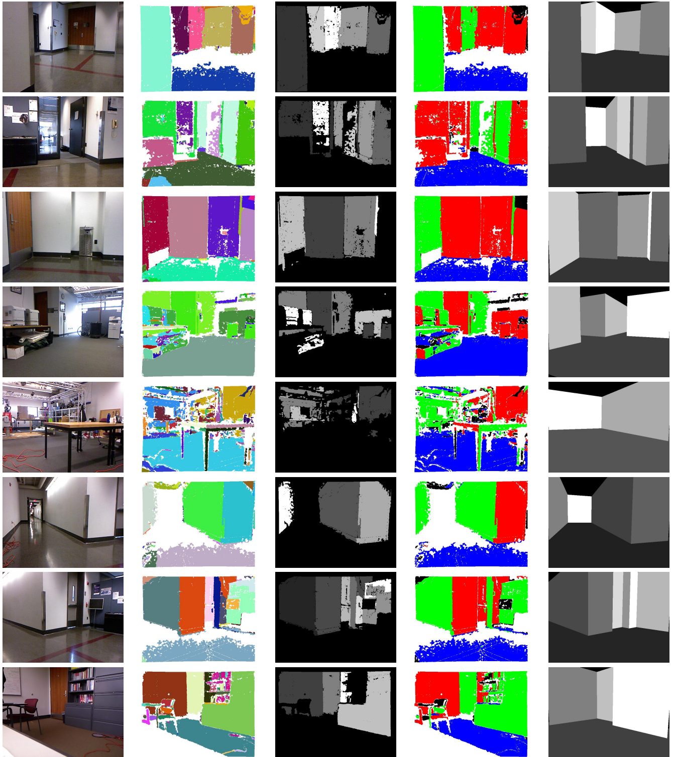
Fig. 8. Figure showing some successful scene parsing results. The second column shows the shows the planar segments extracted from the scene, different colors are used to label points belonging to different planes. The third column shows the points belonging to candidate wall segments, the fourth column shows the results of the analysis that finds the dominant rectilinear structure, Horizontal surfaces are blue and vertical surfaces are red or green depending on their orientation. The final column shows the results of parsing the image into wall segments, each pixel is assigned a label corresponding to the underlying wall.
