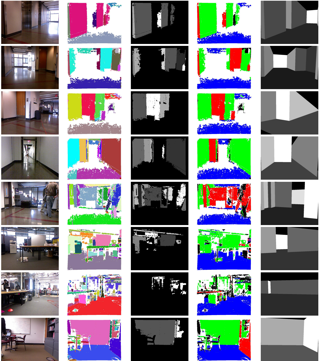
Fig. 9. Figure showing cases where one of the recovered planes has an error. The second column shows the planar segments extracted from the scene, different colors are used to label points belonging to different planes. The third column shows the points belonging to candidate wall segments, the fourth column shows the results of the analysis that finds the dominant rectilinear structure, Horizontal surfaces are blue and vertical surfaces are red or green depending on their orientation. The final column shows the results of parsing the image into wall segments, each pixel is assigned a label corresponding to the underlying wall.
