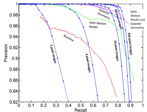
Figure 16. Precision recall curves with a limited field of view equivalent to 0.4% of the original panoramic image (see Figure 6).
