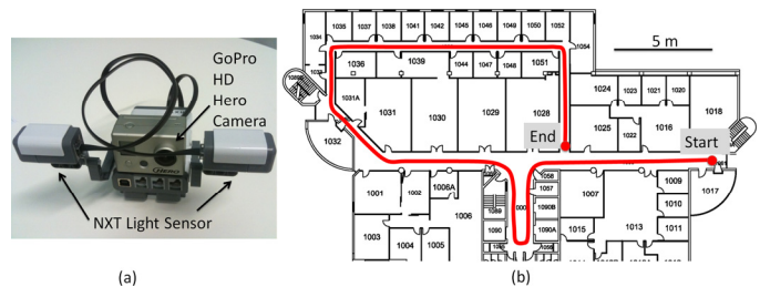
Figure 4. (a) The Lego Mindstorms dataset acquisition rig with 2 sideways facing light sensors and GoPro camera for evaluation of matched routes. (b) The 53 meter long route which was repeated twice to create the dataset.
