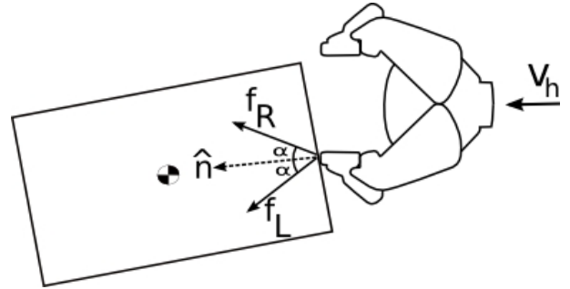
Fig. 3. Notation used for hand-object contacts. The hand’s velocity is given by \mathbf{v}_h . The friction cone edges, (\mathbf{f}_L, \mathbf{f}_R) , and the normal \hat{\mathbf{n}} at the contact are illustrated.
