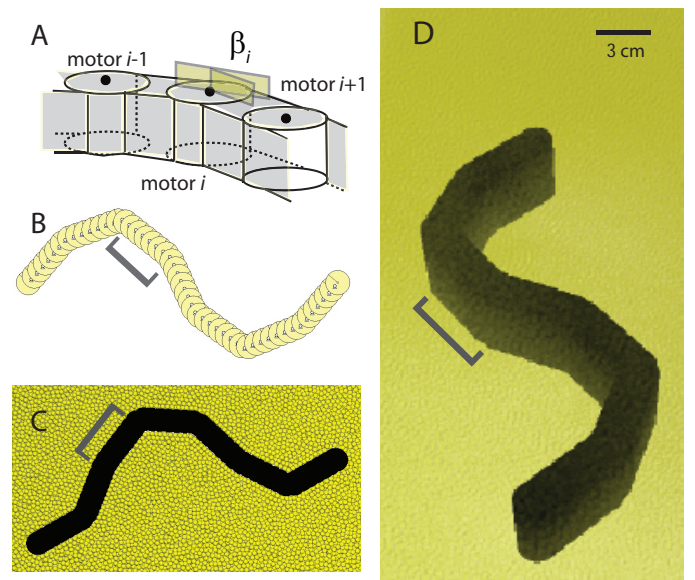
Fig. 3. Simulation of a sand-swimming robot. (A,B) Side and top view of the robot modeled with 49 inter-connected motor segments and one head segment. The angle between adjacent motors ( \beta_i ) is modulated using Eqn. 3 to reproduce the sandfish's sinusoidal traveling wave kinematics. (C) Top view of the device submerged in 6 mm particles with particles above the robot rendered transparent. (D) Rendering of the simulated robot for the same parameters used in robot experiment (see Fig. 4). The brackets ( [ ] ) indicate a single robot segment.
