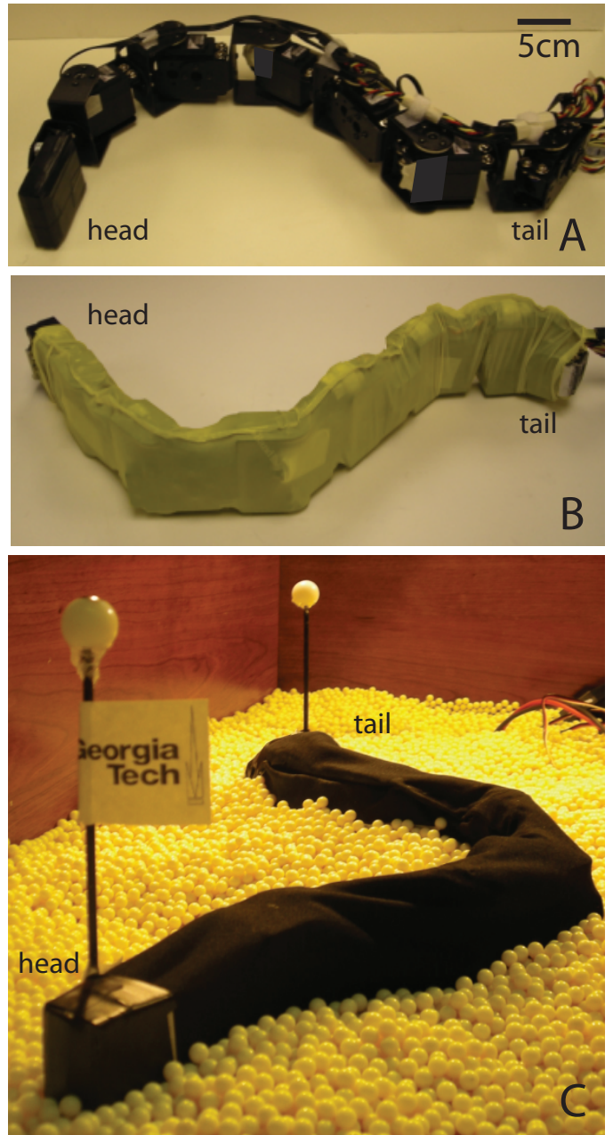
Fig. 4. Prototype of the sand-swimming robot. (A) basic construction (servomotors and aluminium brackets with power wires running along the top of the device). The robot has a double layer skin: (B) tight fitting thin latex inner layer, and (C) Lycra spandex outer layer. Balls on narrow masts on the head and tail segments allow subsurface motion tracking.
