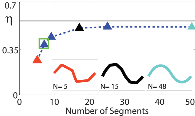
Fig. 8. Wave efficiency increases with number of segments for a fixed length robot in simulation (blue dashed curve) ( f = 1 Hz and A/\lambda = 0.2 ). The red, black, and cyan triangles correspond to 5, 15, and 48 segment robots respectively. The green square corresponds to the seven segment physical robot, and the grey line indicates \eta predicted by the RFT solved for a continuous body profile (see text for details).
