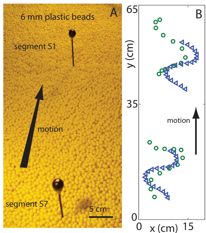
Fig. 6. Subsurface swimming in experiment and simulation. (A) Robot submerged in a container filled with 6 mm plastic particles. Masts with spherical markers are attached to the first and last module. (B) Kinematics of the first and last segment of the robot in experiment (green circles) and simulation (blue triangles).
