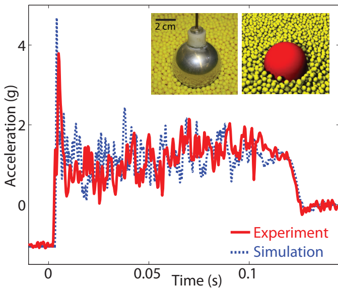
Fig. 2. Validation of the multi-particle discrete element method (DEM) simulation of the granular medium using measured acceleration of a sphere during vertical impact after free-fall. Acceleration vs. time in simulation (blue dashed trace) and experiment (red solid trace) agree well. The impact velocity for this representative run is 1.4 m/s. Acceleration is in units of g , the acceleration due to gravity. (Left inset) Aluminium ball instrumented with accelerometer resting on 6 mm plastic particles. (Right inset) Ball and particles in simulation.
